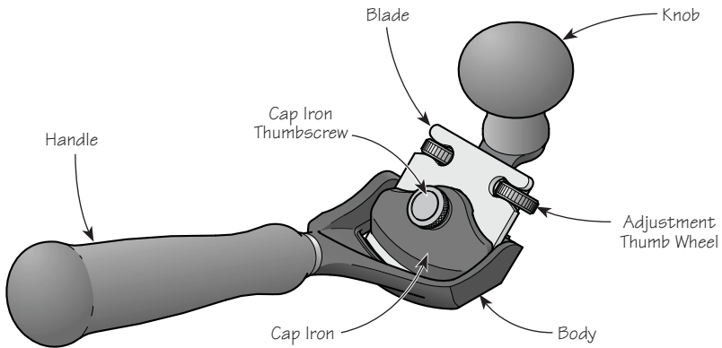
Figure 1: Pullshave components.
